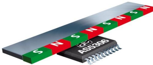
Figure 1: Arrangement with multi-pole strip magnet
